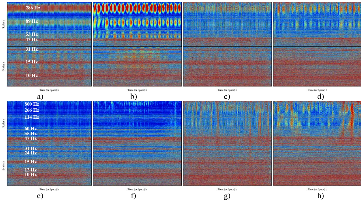
Fig. 3. Wavelet spectrograms of acceleration signal in cutting direction for as-cast HCCI with low C-Si content at different feed rates: BCBN tool a) 0.1 mm/rev, 5 revolutions; b) 0.5 revolutions; c) 0.6 mm/rev, 5 revolutions; d) 0.5 revolutions; HCBN tool e) 0.1 mm/rev, 5 revolutions; f) 0.5 revolutions; g) 0.6 mm/rev, 5 revolutions; h) 0.5 revolutions.
