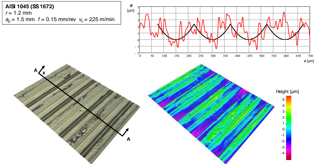
Fig. 2. Obtained surface micro topography while longitudinally turning AISI 1045, (Schultheiss, 2013). The 2D-graph illustrates the measured (red) and theoretical surface roughness, Equation 2 (black).
