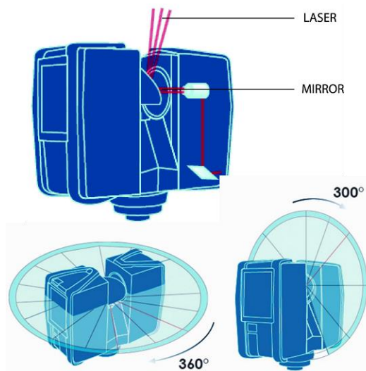
Fig. 1. 3D laser scanning capturing (FARO Technologies, 2013).
